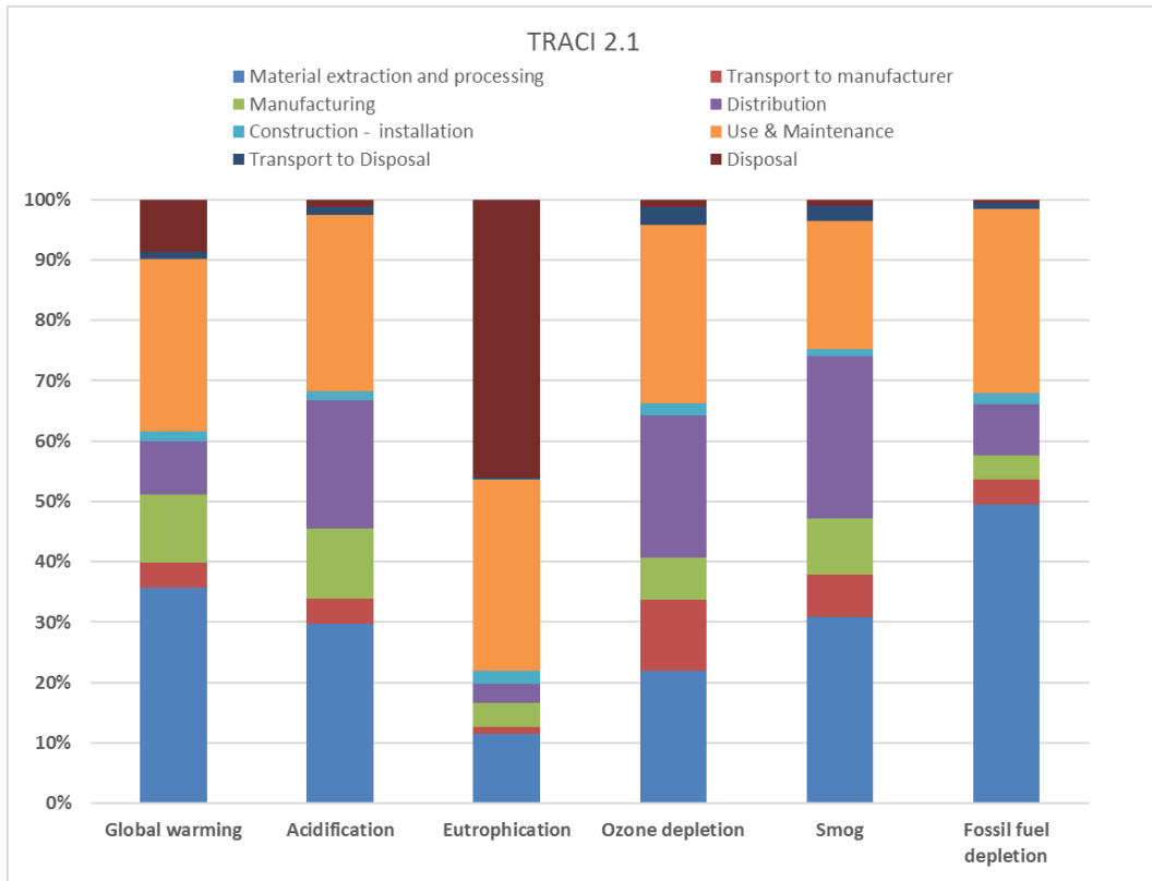
Figure 2. Contribution analysis for the Aspecta Tilt & Tones ISOCORE LVT product system – TRACI v2.1.
