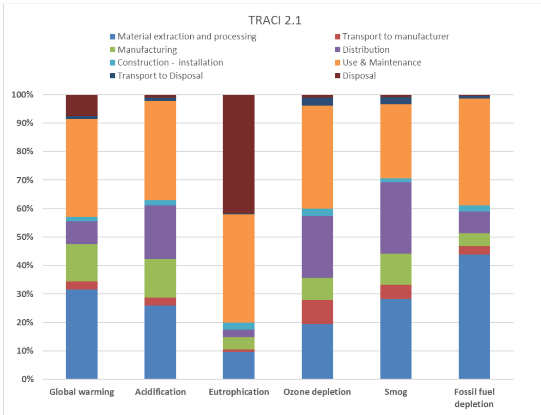
Figure 4. Contribution analysis for the Elemental ISOCORE 6.5 mm LVT product system – TRACI v2.1.
